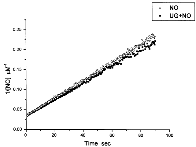
Figure 8. Auto-oxidation of 30 \mu\text{M} nitric oxide (NO) in PBS in the absence or presence of cat's claw extract (UG, 5 mg/mL) pH 7.4 at 25 ^{\circ}\text{C} . Open circles indicates NO concentration degradation. Closed squares (UG + NO) degradation of NO in the presence of cat's claw extract. Nitric oxide was recorded continuously as described in Materials and Methods. Slope of the two lines indicates that half-life of NO was not affected significantly. Data are from three experiments, each performed in triplicates.
