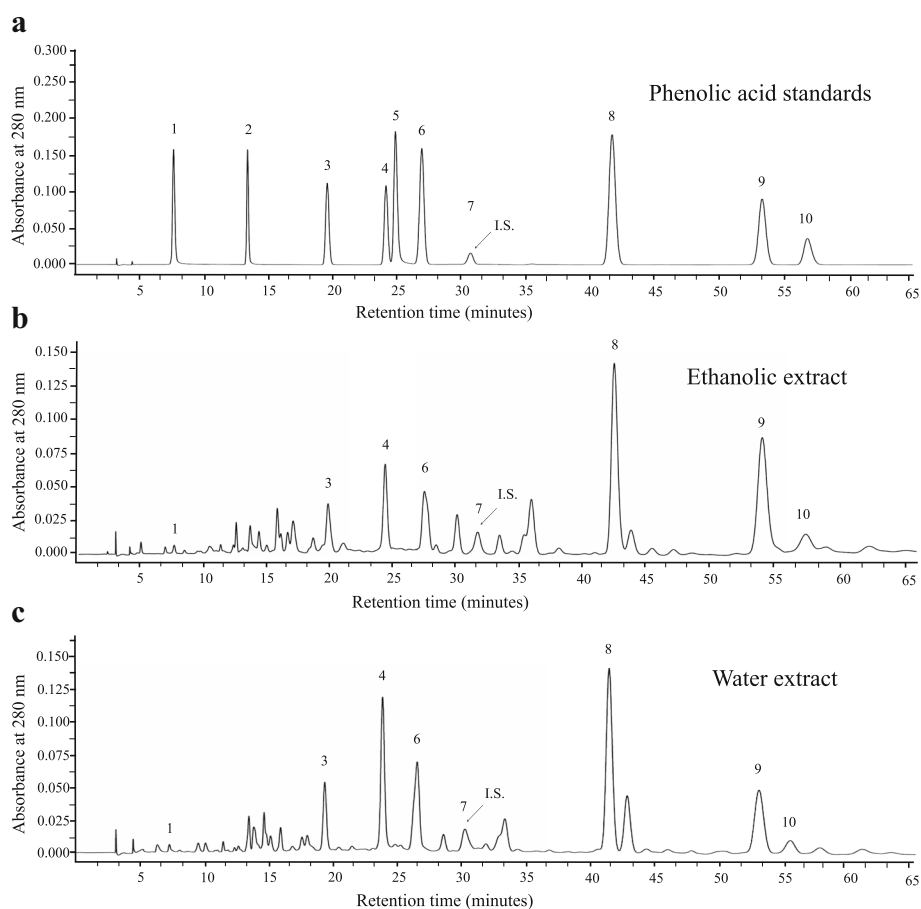
Fig. 7 HPLC chromatograms of phenolic acid standards ( a ), base hydrolyzed ethanolic ( b ) and water ( c ) extracts of the powdered formula of H. cordata fermented broth and P. emblica fruit where 1 = gallic acid, 2 = protocatechuic acid, 3 = p -hydroxybenzoic acid, 4 = vanillic acid, 5 = caffeic acid, 6 = syringic acid, 7 = p -hydroxybenzaldehyde, 8 = p -coumaric acid, 9 = ferulic acid and 10 = sinapinic acid. p -Hydroxybenzaldehyde was used as an internal standard (I.S.)
