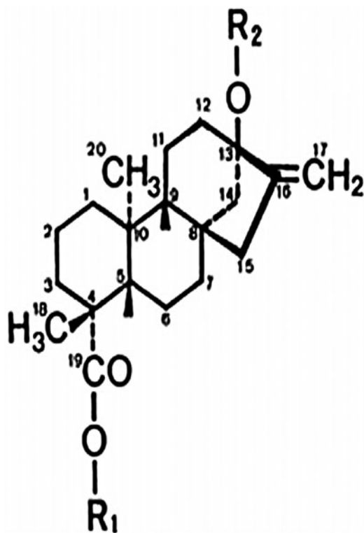
FIG. 3. Chemical structure of the steviol molecule.
